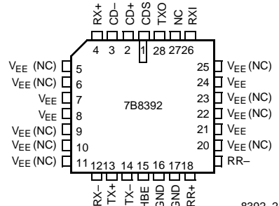
PLCC Top View
