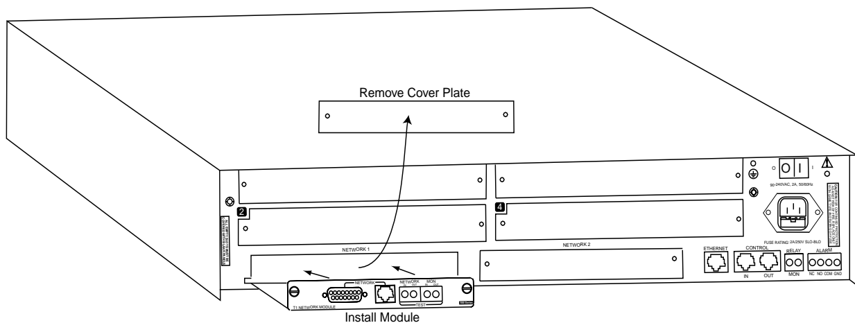
Figure 1. Installing the T1 Network Interface Module
